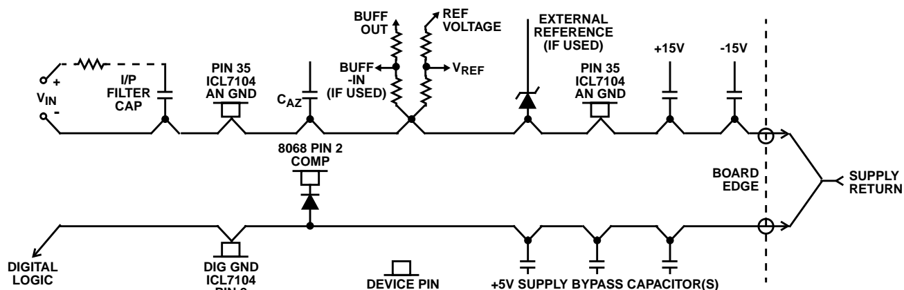
FIGURE 16. GROUNDING SEQUENCE
