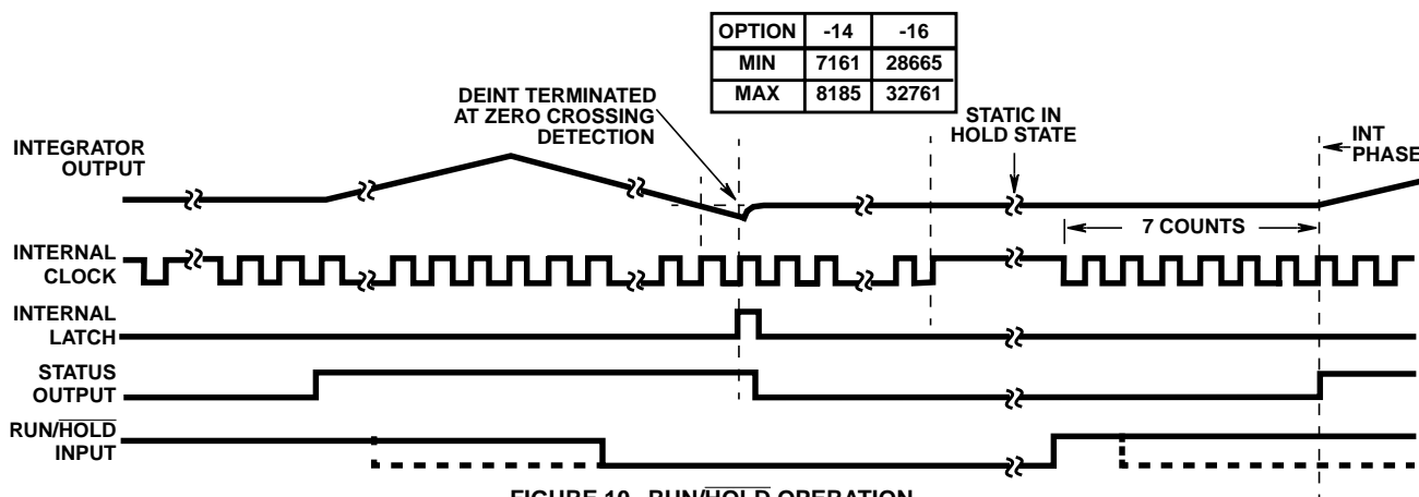
FIGURE 10. RUN/HOLD OPERATION
